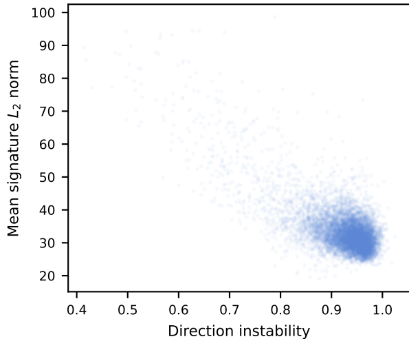
(a) Instability vs. signal strength ( \rho = -0.41 )
