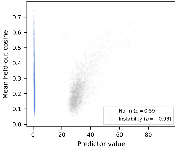
(b) Norm vs. instability as predictors
