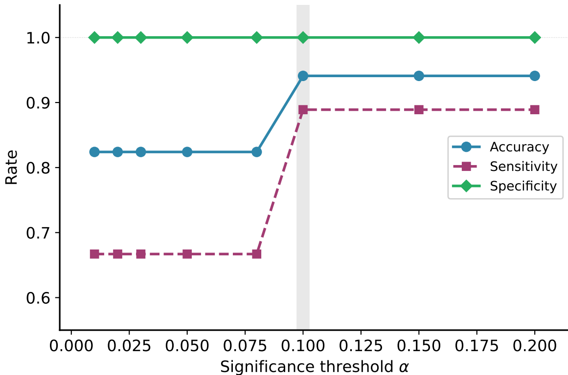
Sensitivity analysis across classification thresholds
