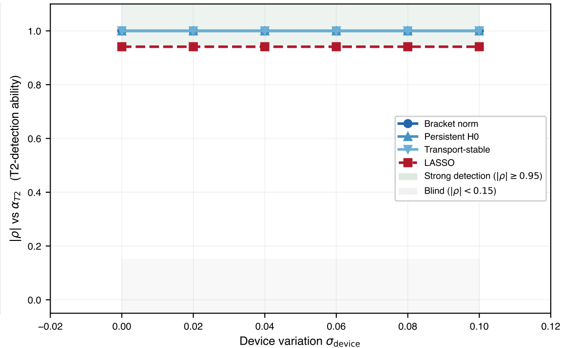
Can methods detect T2 decoherence as device variation increases?
