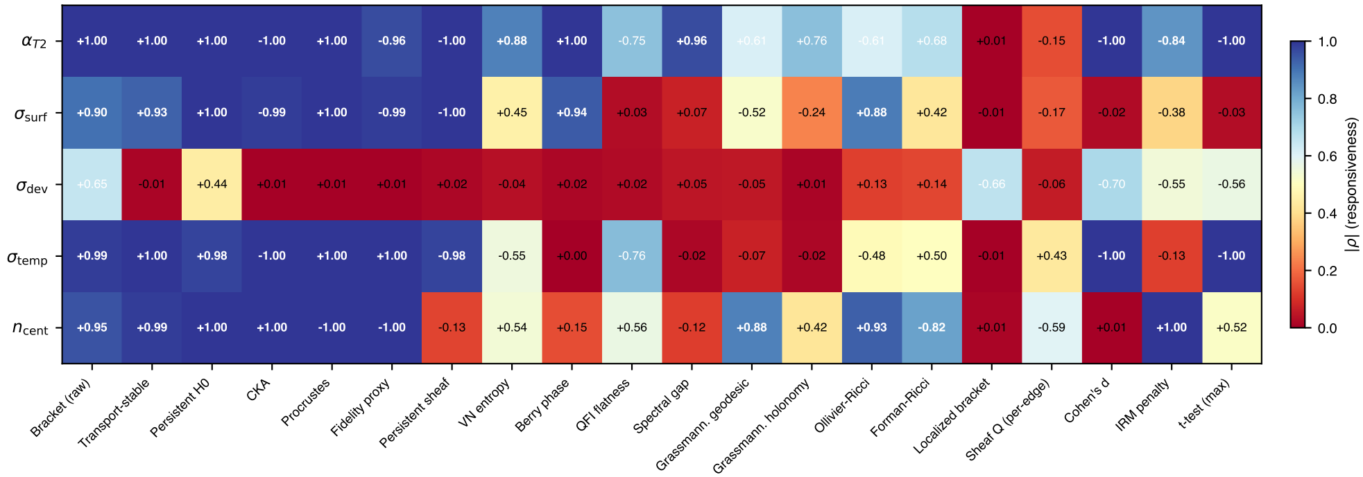
Method--axis sensitivity map (median Spearman \rho , 100 seeds)
