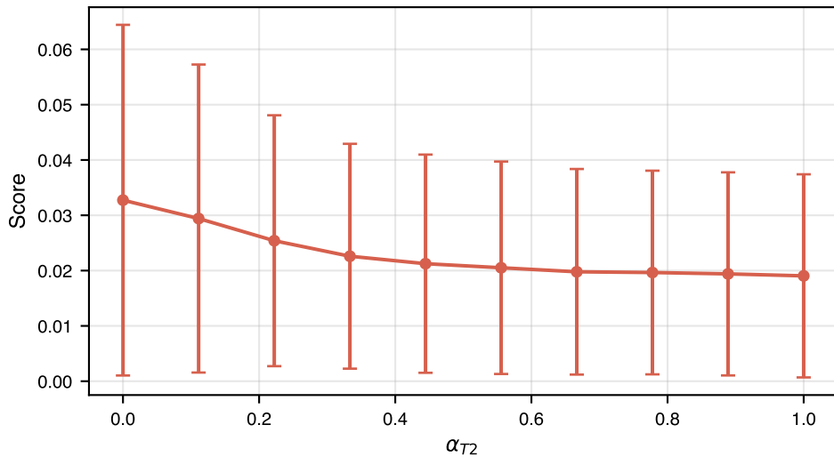
Sheaf H^1 (Cochran's Q) ( \rho = -0.15 )
