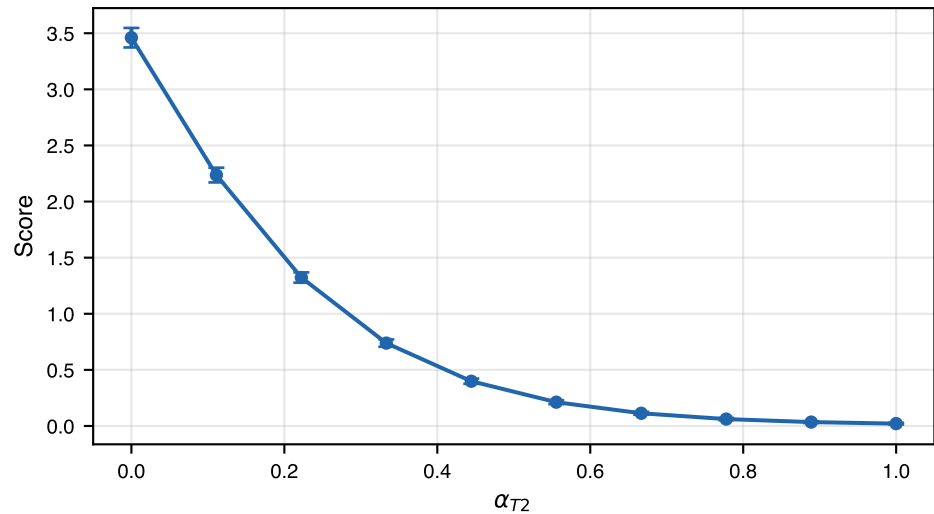
Persistent sheaf cohomology ( \rho = -1.00 )
