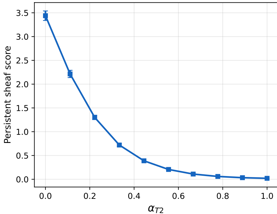
Persistent sheaf: monotonic ( \rho = -1.00 )
