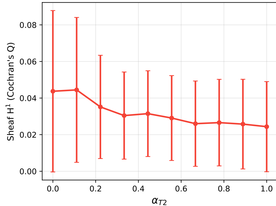
Pointwise sheaf H^1 : flat ( \rho = -0.29 )
