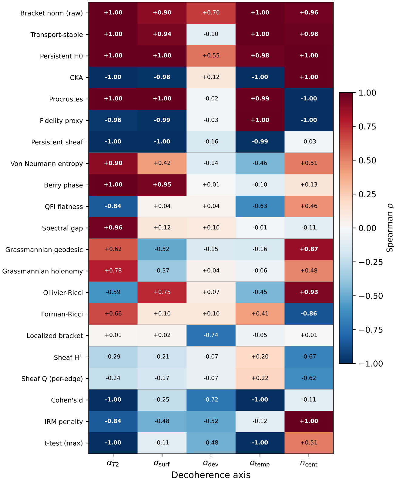
Method--axis sensitivity map (median Spearman \rho , 20 seeds)
