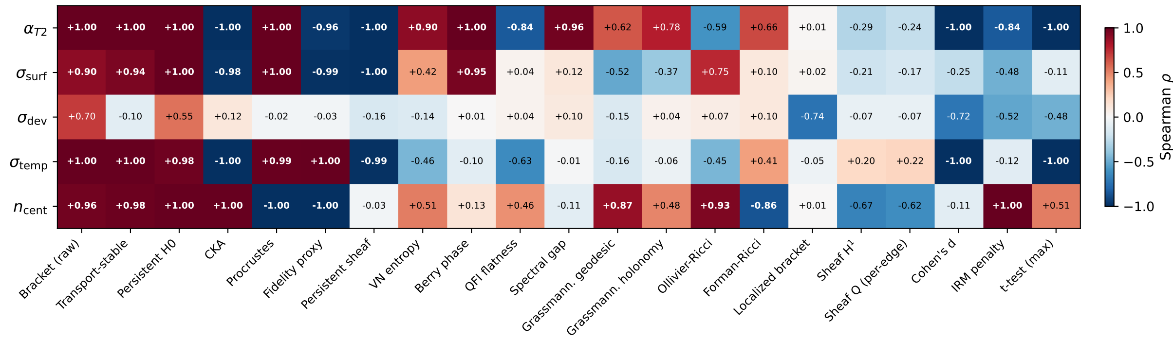
Method--axis sensitivity map (median Spearman \rho , 20 seeds)
