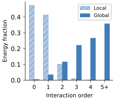
(a) Cell cycle transcription \Delta_{3+} = +83.2\text{pp}
