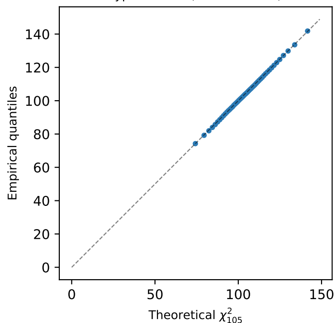
K=8, d=15 (df=105) Type I: 0.049 (nominal: 0.05)
