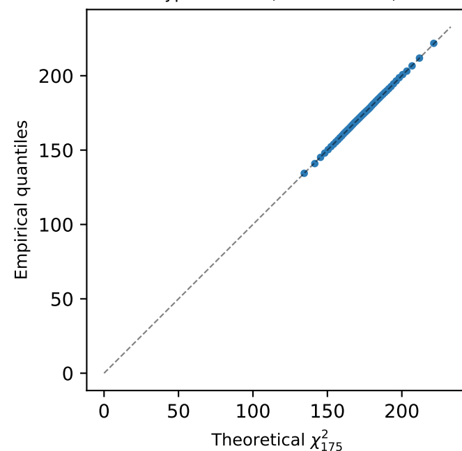
K=8, d=25 (df=175) Type I: 0.049 (nominal: 0.05)
