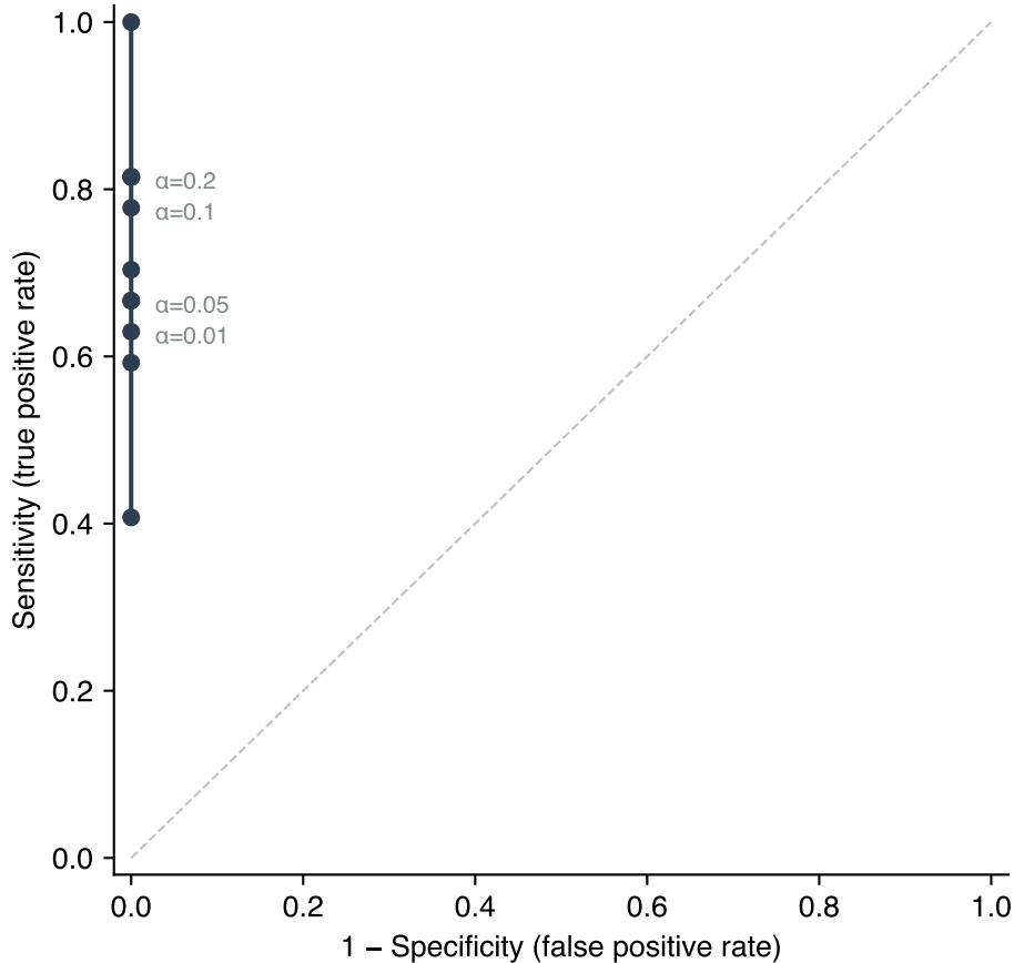
Q-test classification across a thresholds
