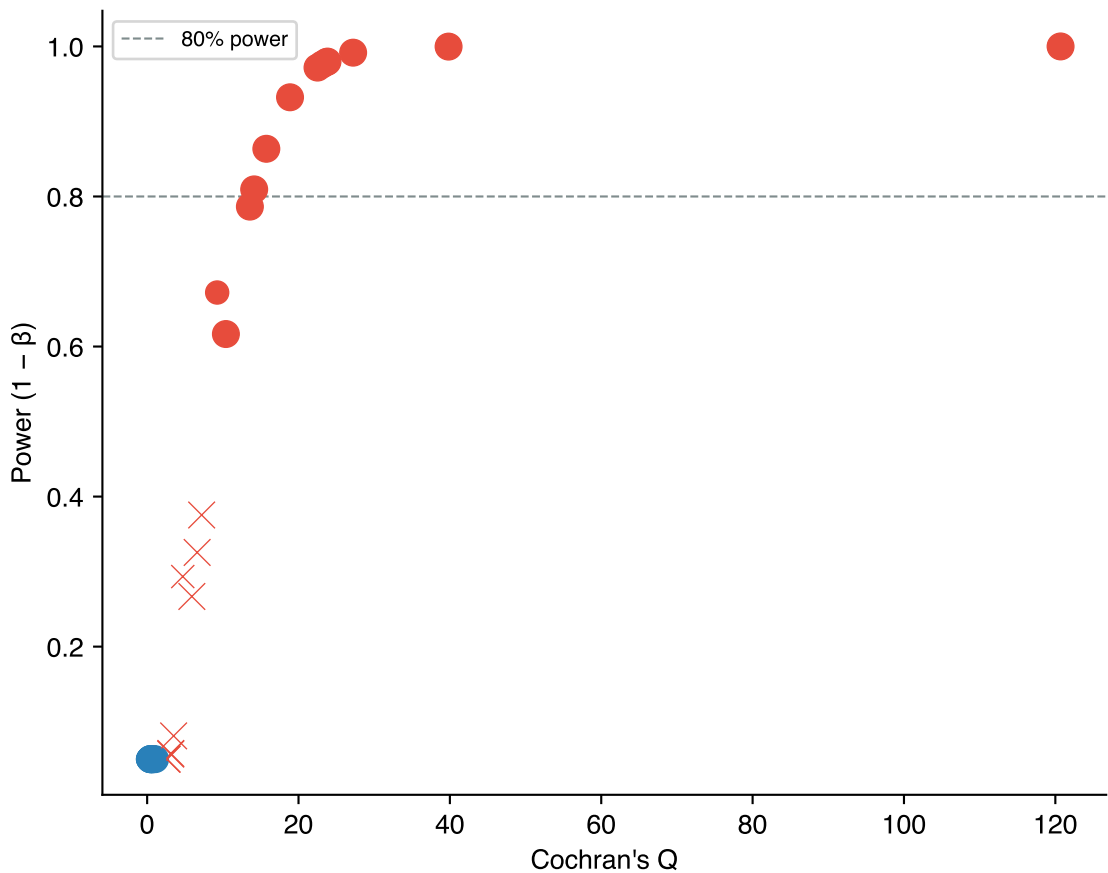
Power vs Q statistic
