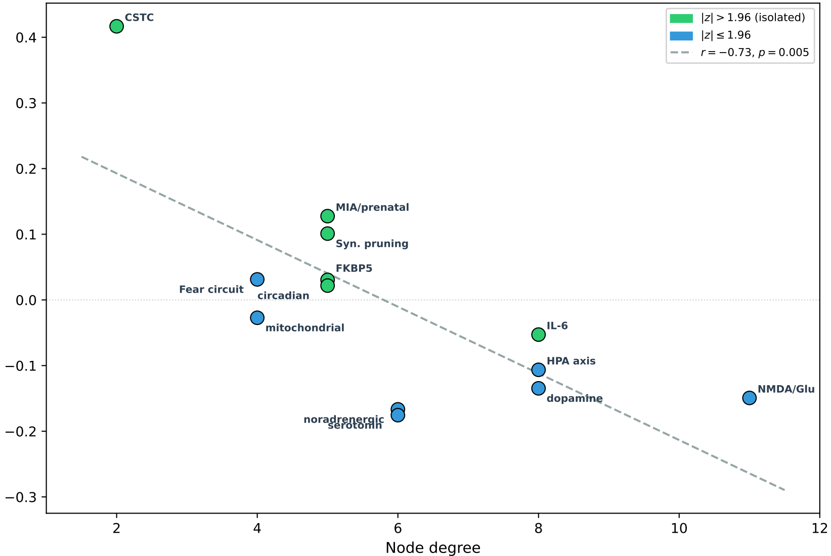
Mean Ollivier-Ricci curvature
