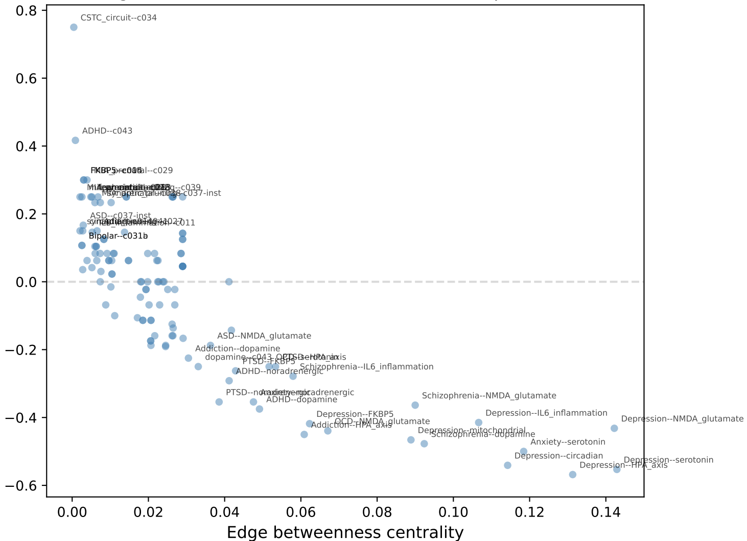
Edge betweenness vs curvature ( r = -0.787 , \rho = -0.713 )
