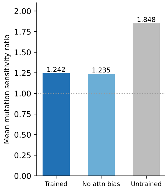
A. Mean ratio
