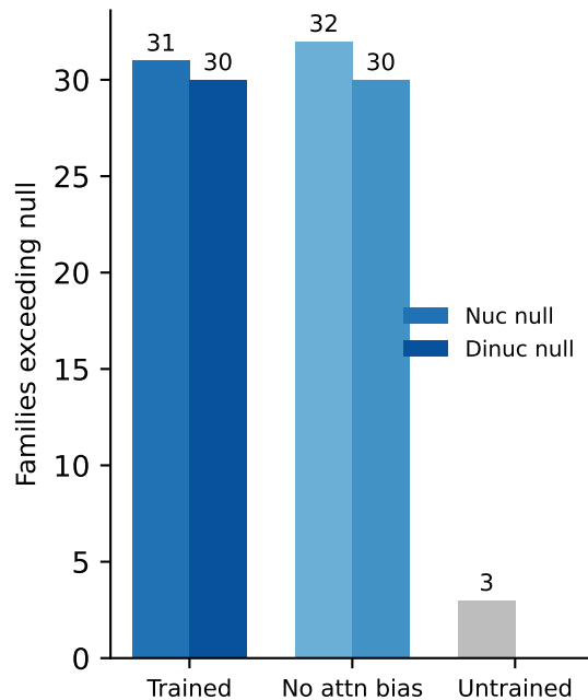
B. Exceedance counts
