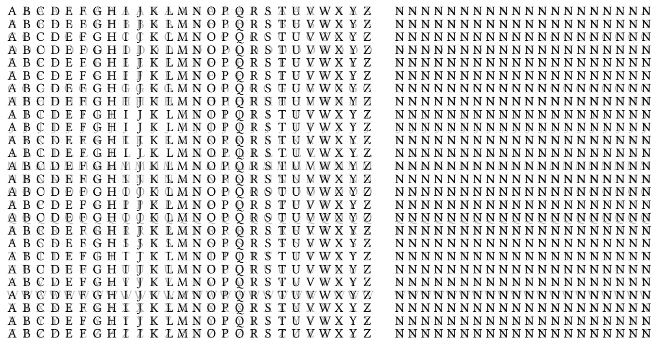
Figure 3: Above-anchor X coordinate alignment. In the left panel, the 26×26 grid shows letters A–Z aligned at the their above-anchor. The right panel shows how hard it is to discern bad X coordinates. The right panel shows N aligned with letters at their above-anchor, starting at the first column with Ns above-anchor as currently set by the font, and then spoofing increasing bad values for the X coordinate of N's above-anchor, by 5 UPM per column. At the rightmost column, it becomes evident that the (spoofed) X coordinate of N's above-anchor is bad, because in that column the black Ns are too far right of the gray letters below them.
