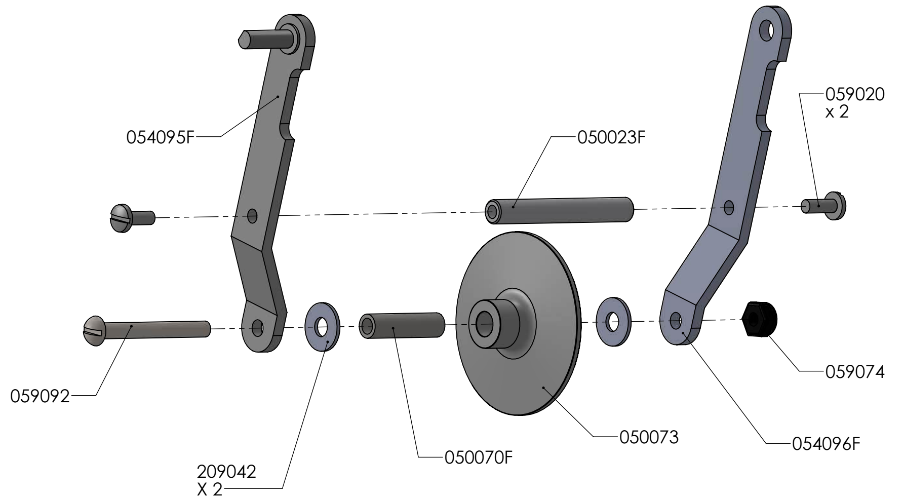
CREASER ASSY
