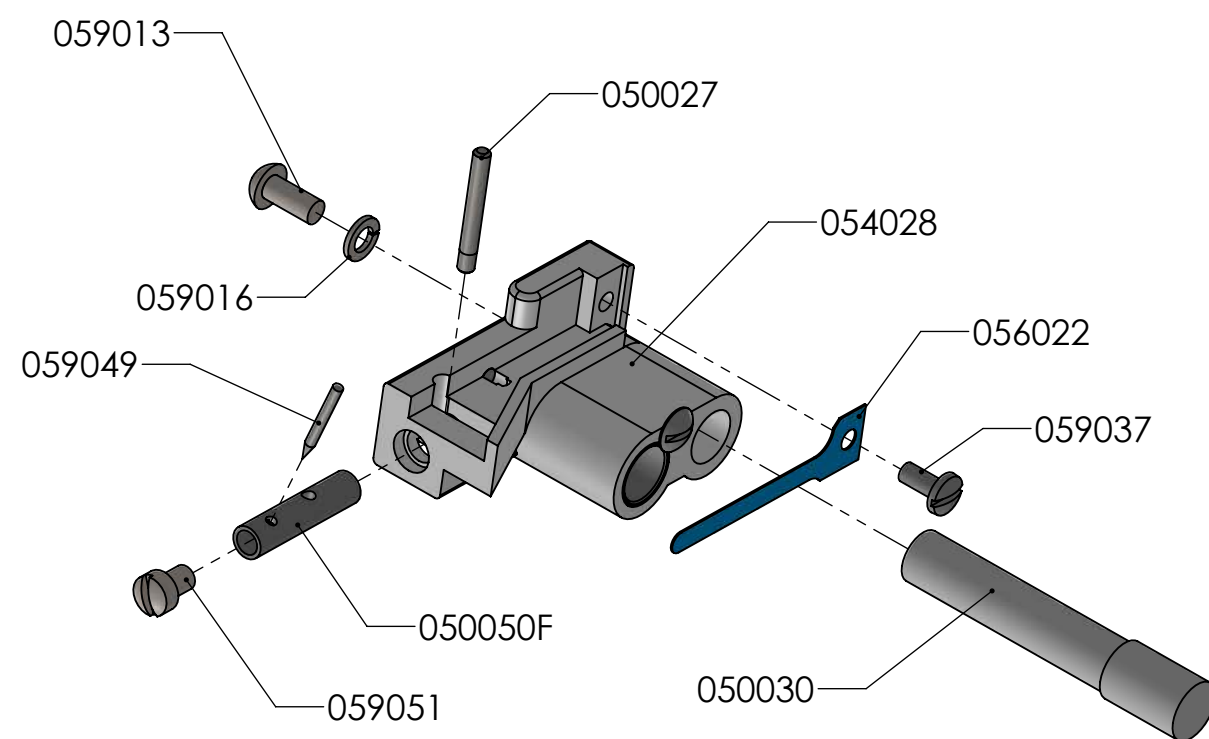
GOOSER ASSY
