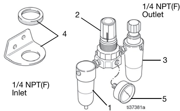
Model 110149, Series A Includes items 1-5
