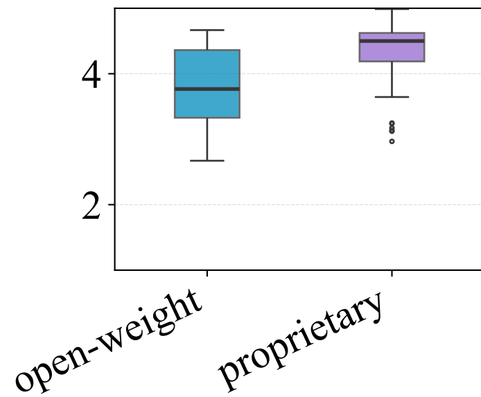
Conscientiousness
