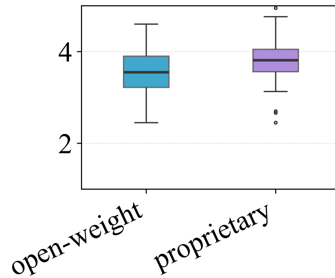
Extraversion
