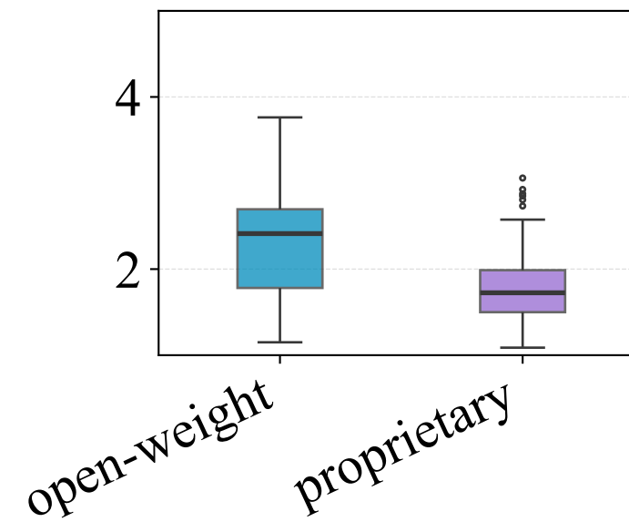
Neuroticism
