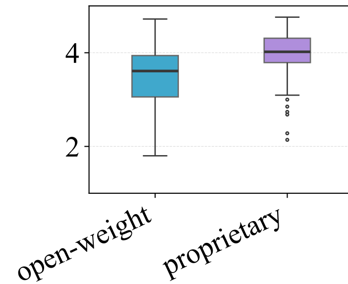
Openness
