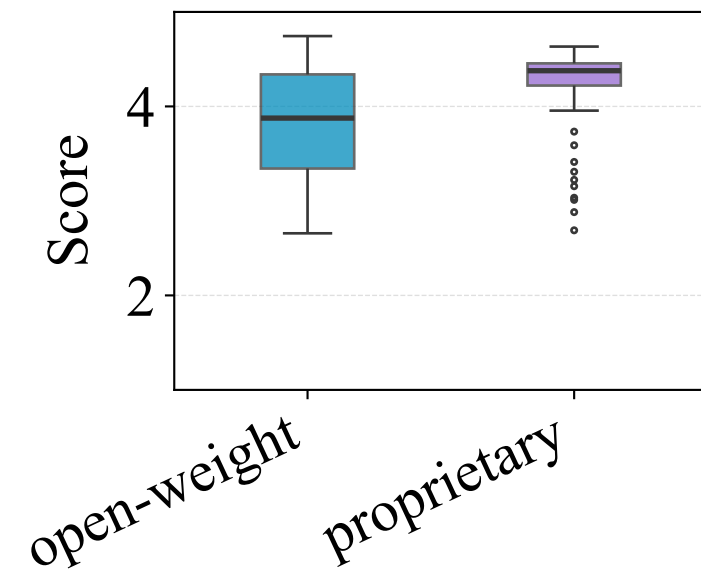
Agreeableness
