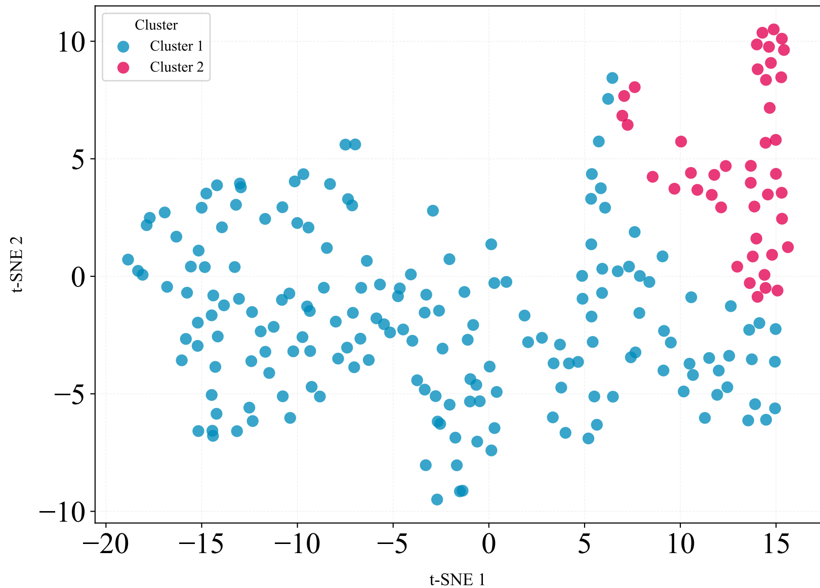
t-SNE — Item Response Space (k=2 clusters)
