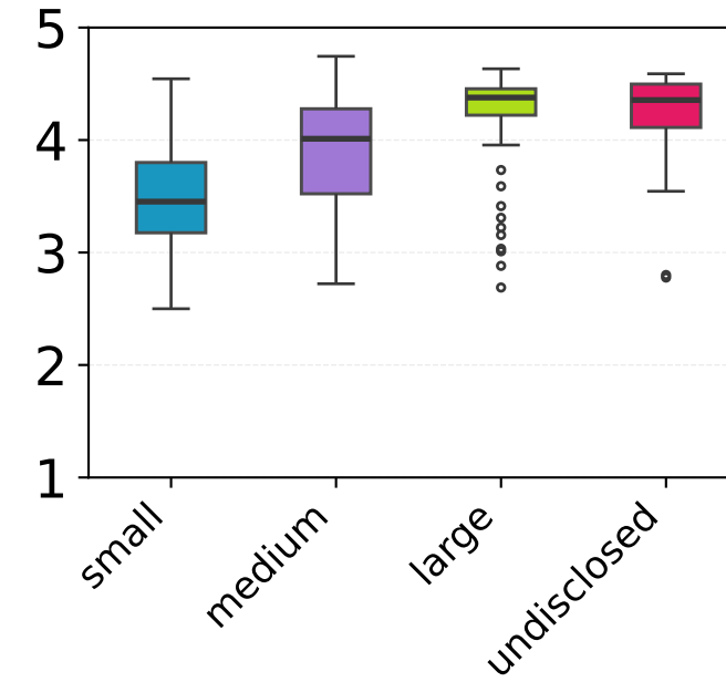
Agreeableness
