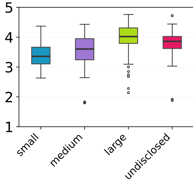
Openness
