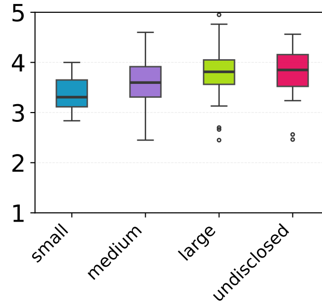
Extraversion
