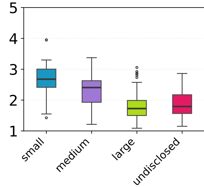
Neuroticism
