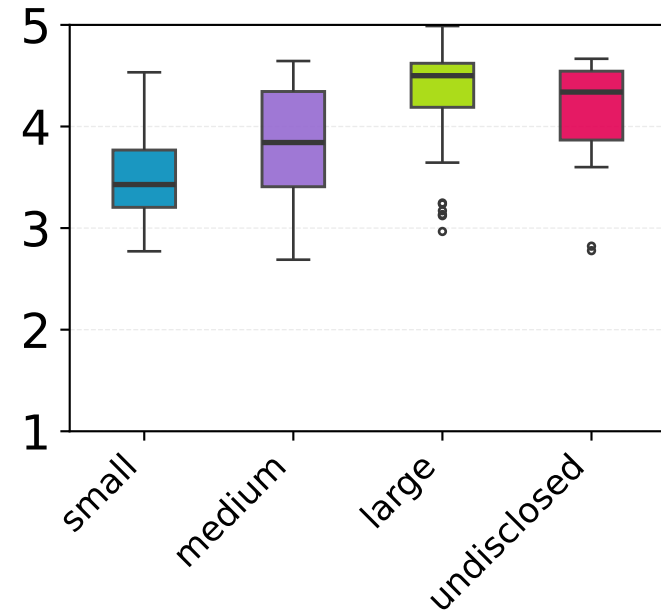
Conscientiousness
