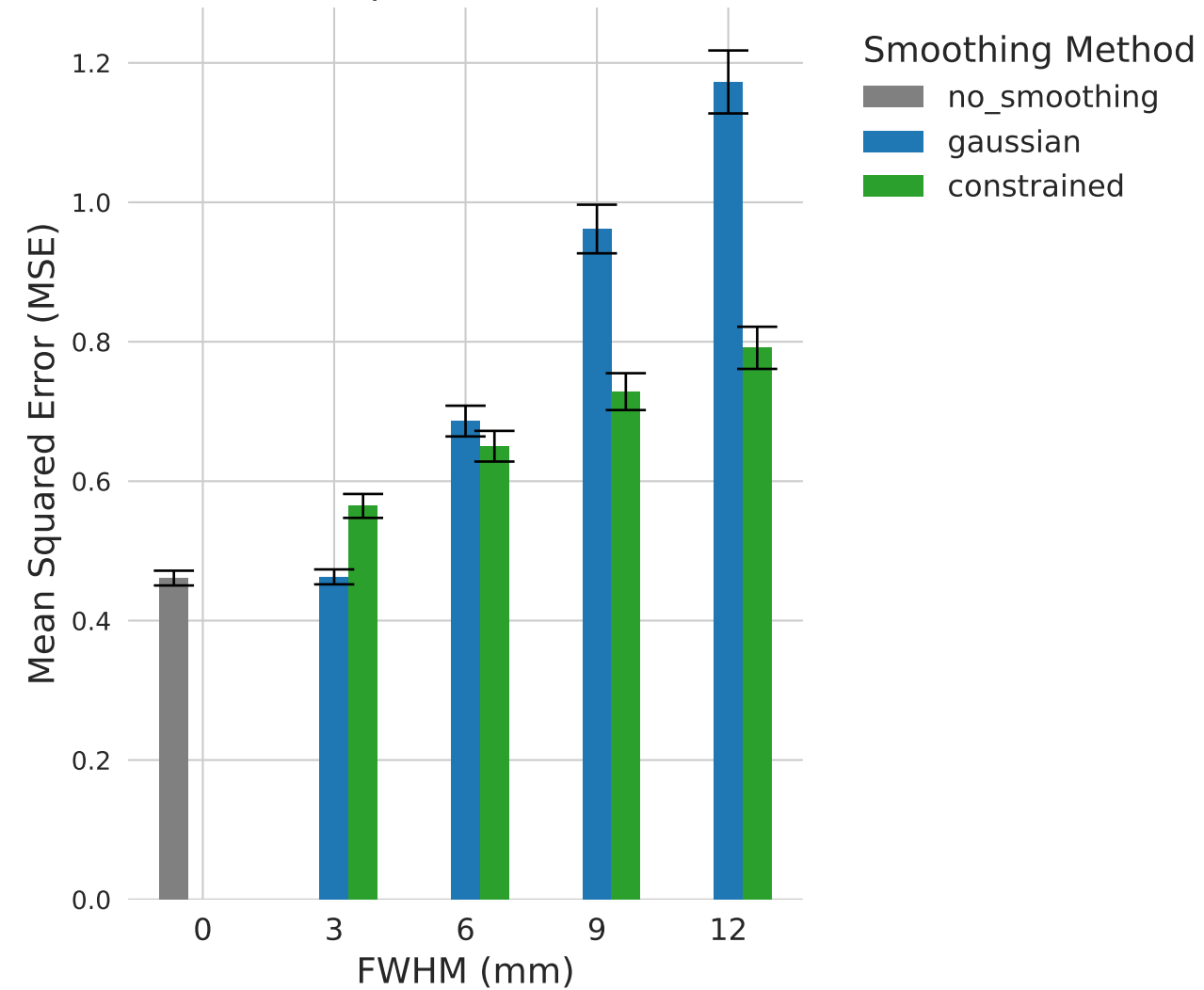
Mean Squared Error (MSE)
