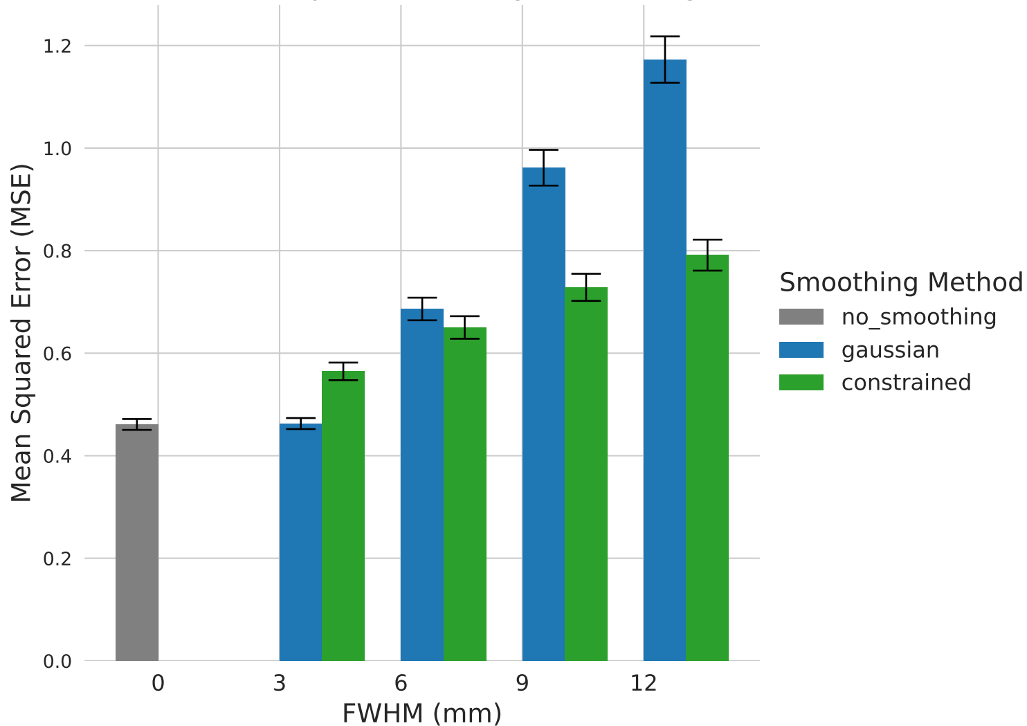
Motor Task Mean Squared Error by Smoothing Method
