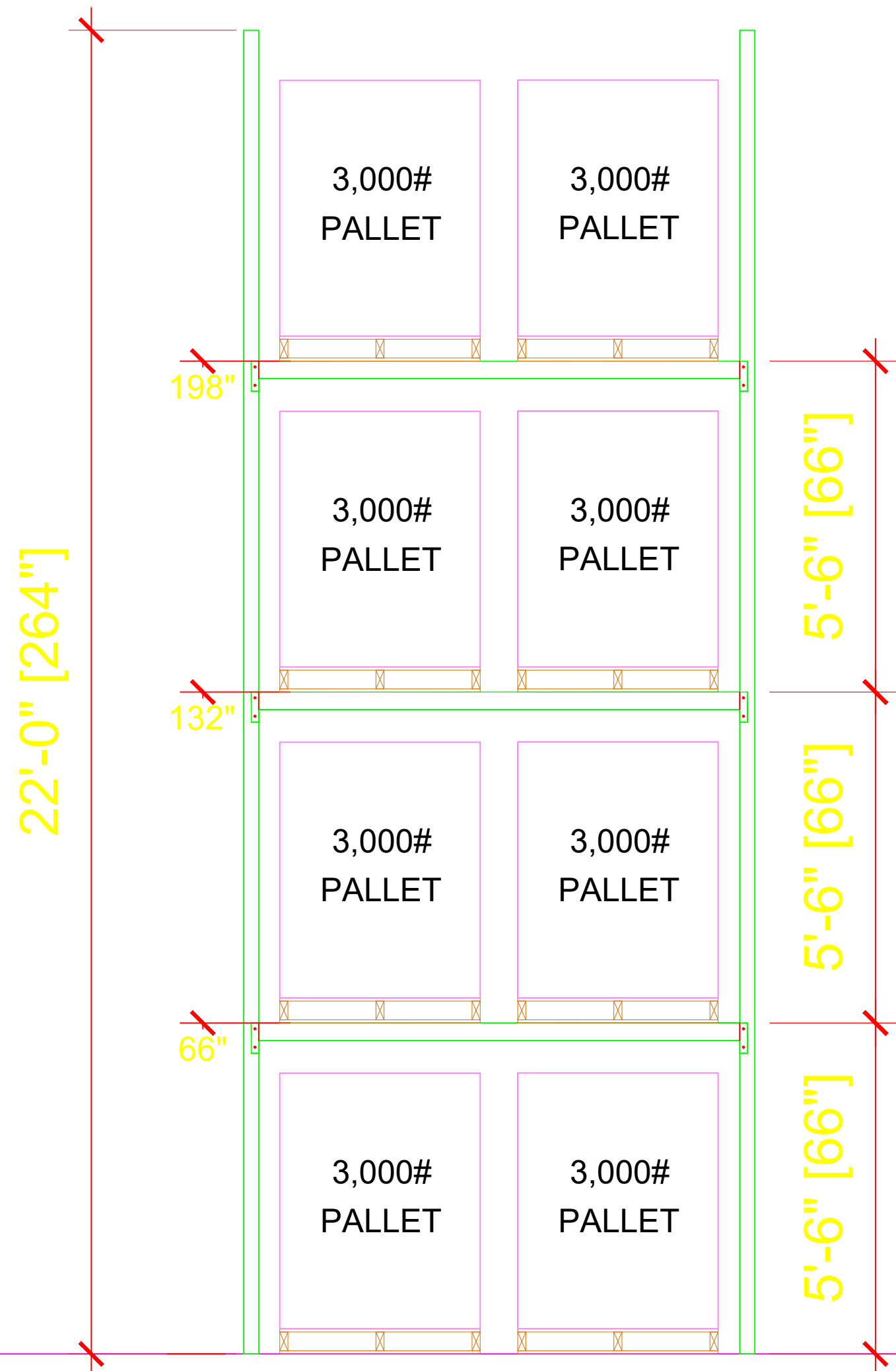
RACK ELEVATION
