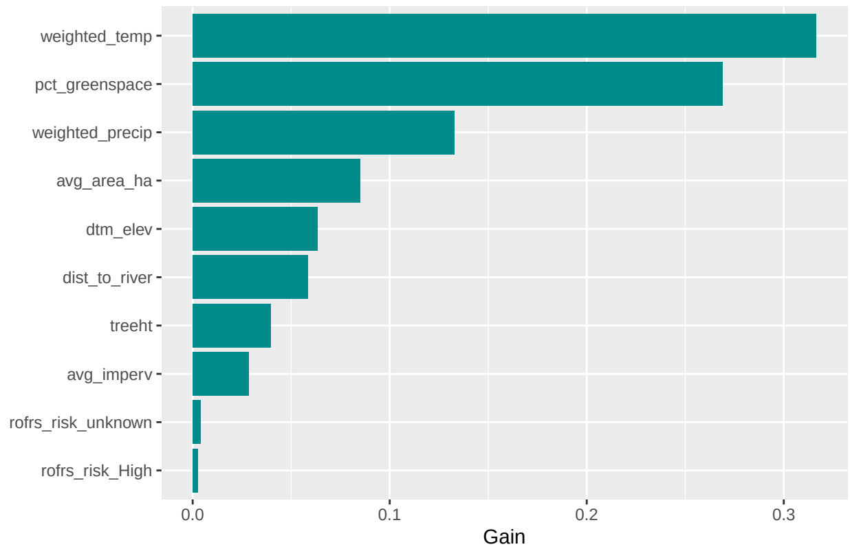
Variable importance: ND species richness classification (XGBoost)
