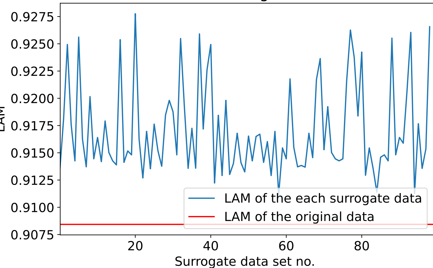
LAM of the each surrogate data for m=3
