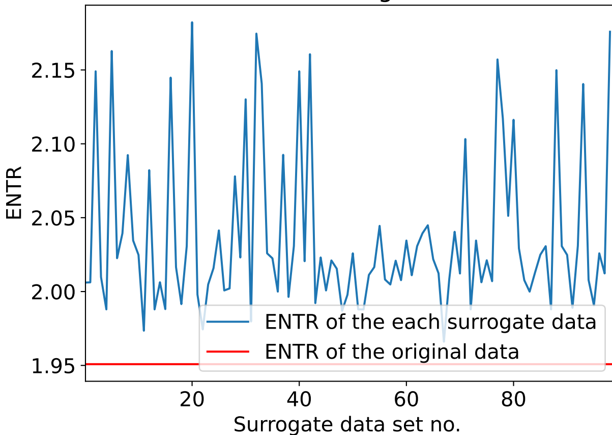
ENTR of the each surrogate data for m=3
