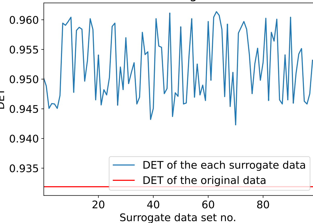
DET of the each surrogate data for m=6
