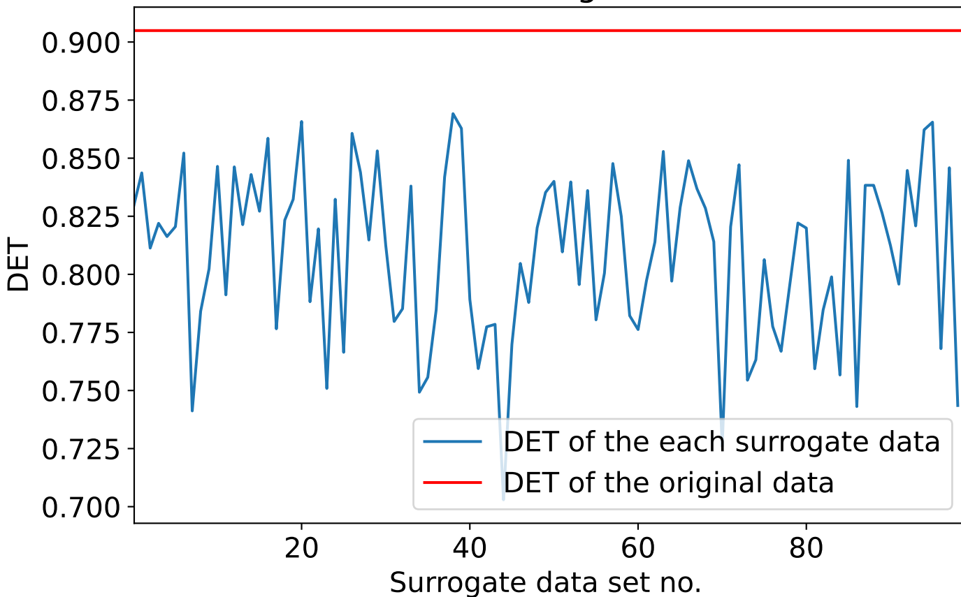
DET of the each surrogate data for m=5
