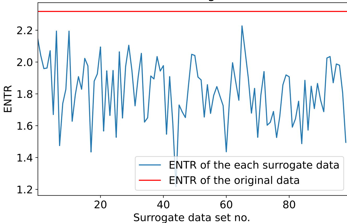
ENTR of the each surrogate data for m=6
