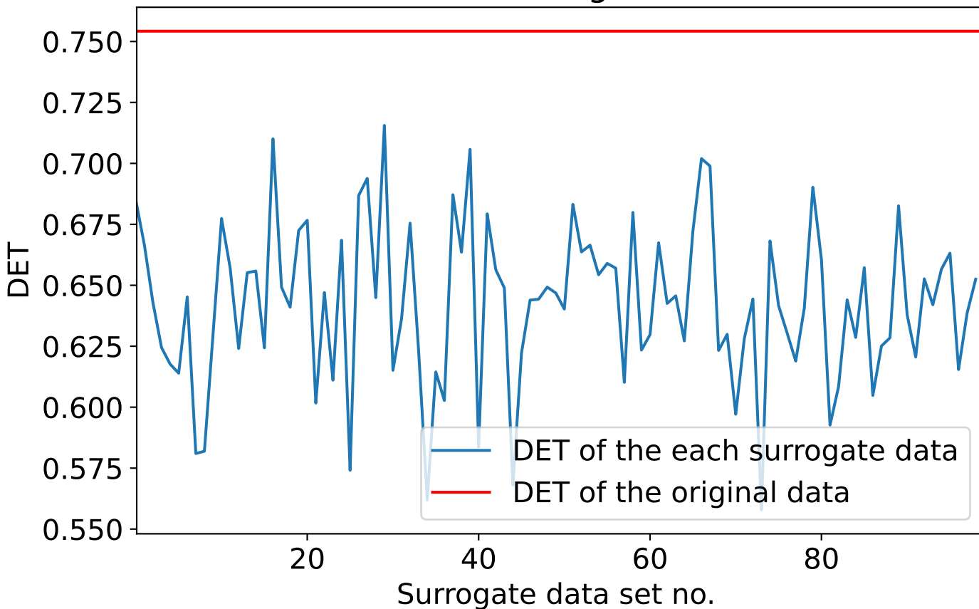
DET of the each surrogate data for m=2
