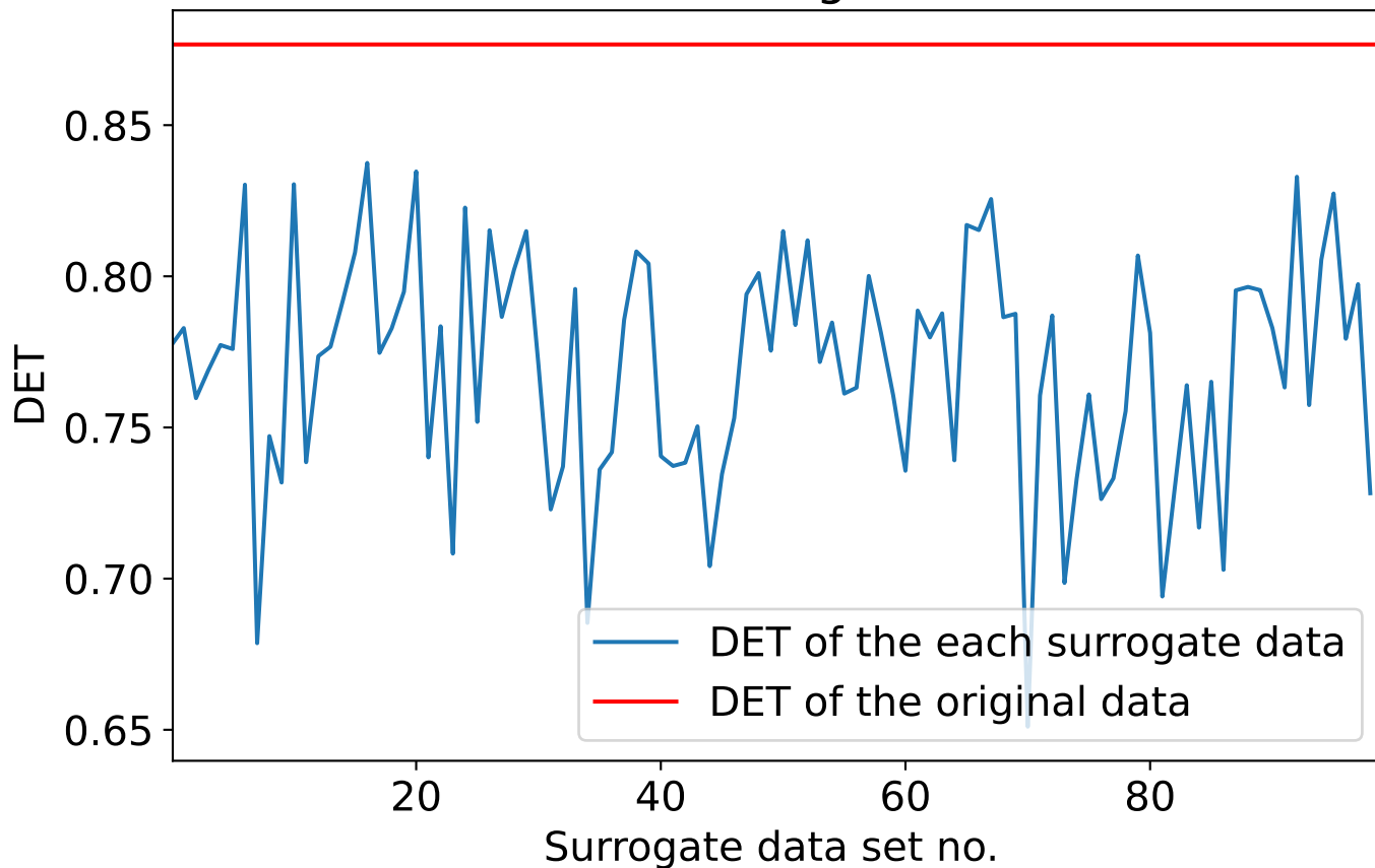
DET of the each surrogate data for m=4
