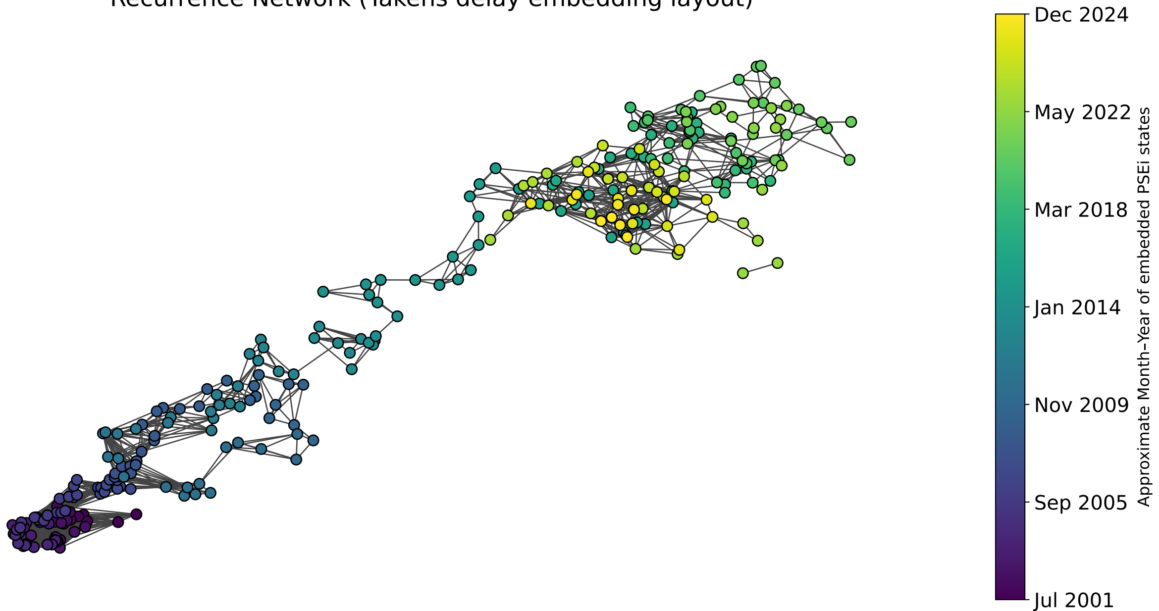
Recurrence Network (Takens delay embedding layout)
