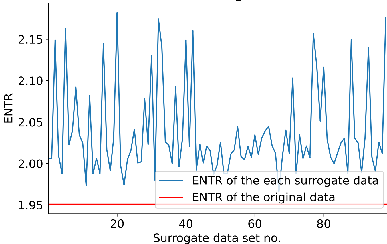
ENTR of the each surrogate data for m=3
