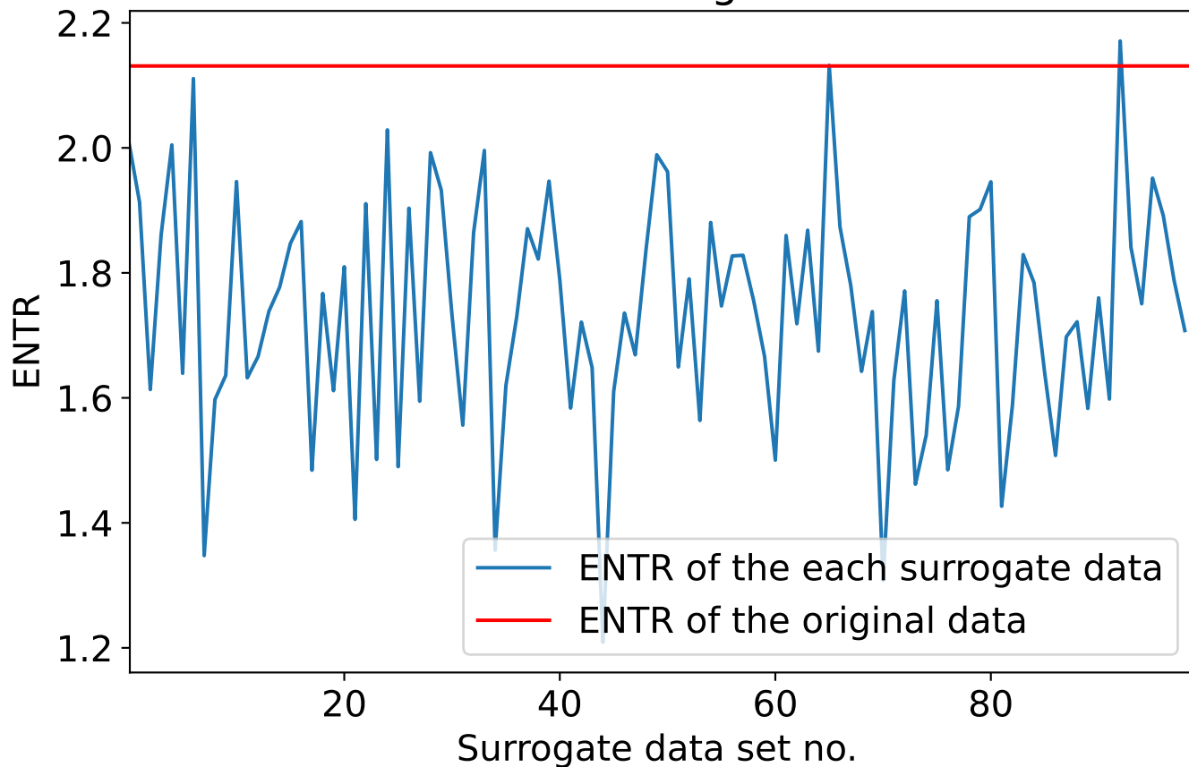
ENTR of the each surrogate data for m=5
