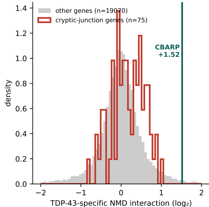
C · Exploratory NMD interaction (four condition-level units)
