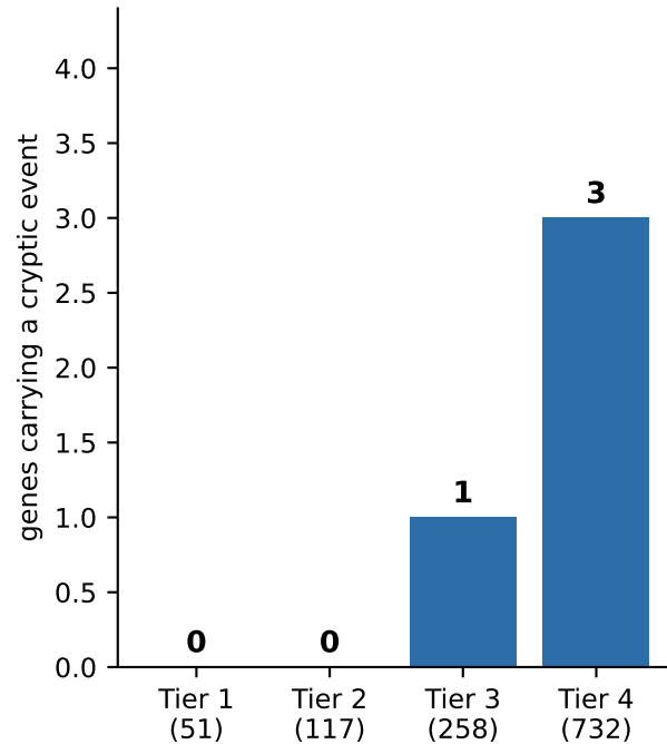
B · Cryptic events in the Ca 2+ panels (none in the core SOCE/TRP set)
