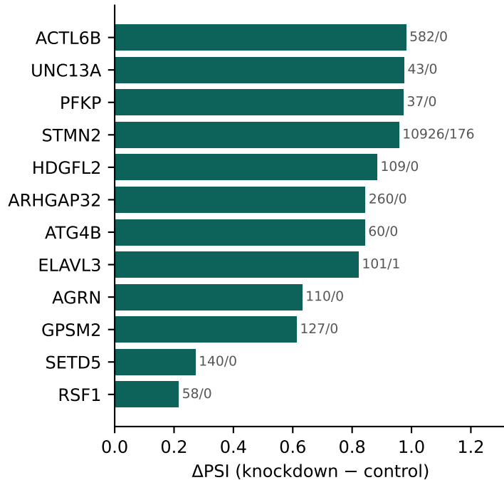
A · Cryptic positive controls, recovered de novo (read counts KD/control)
