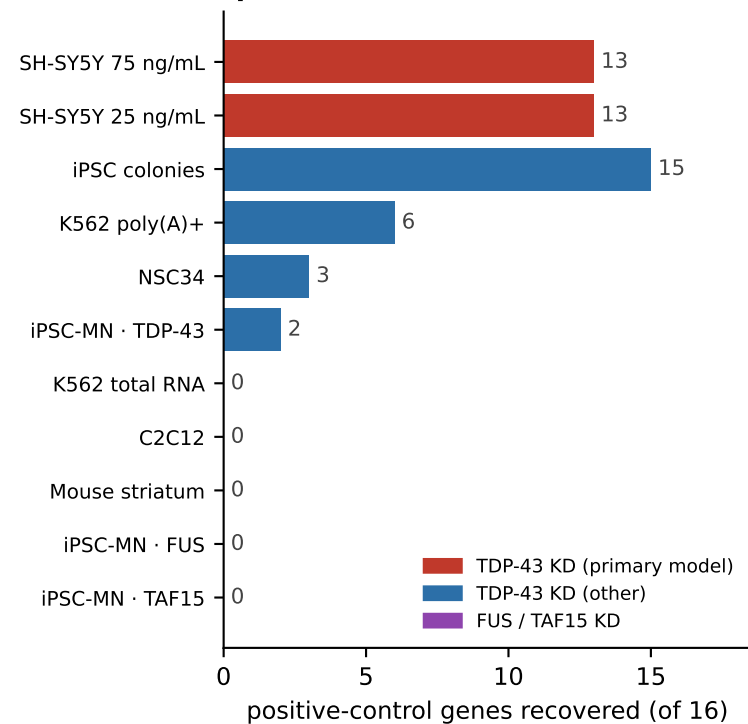
A · Positive-control recovery by comparison (permissive definition)
