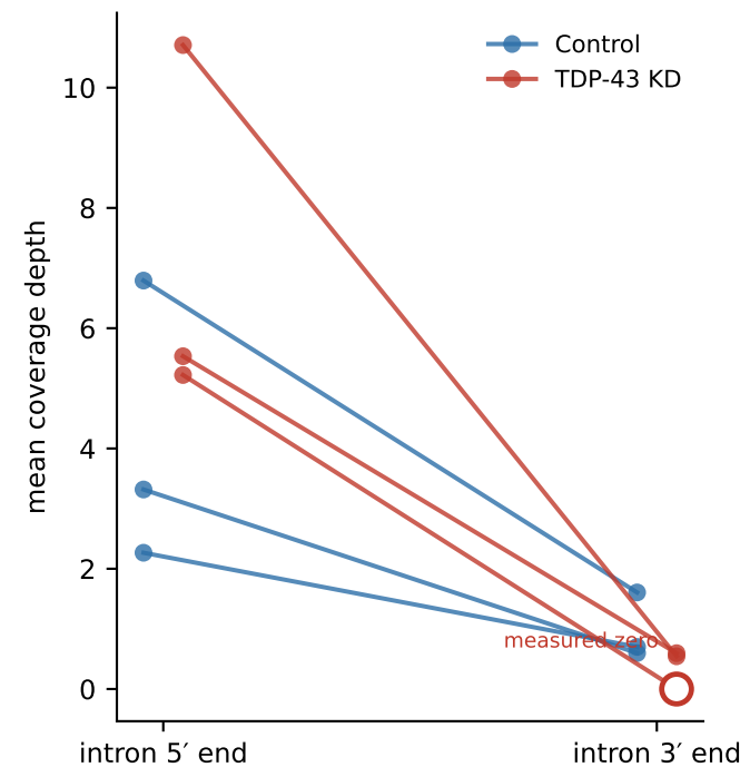
C · Corrected coverage across STMN2 intron 2 (one knockdown 3' window has a measured coverage of zero)
