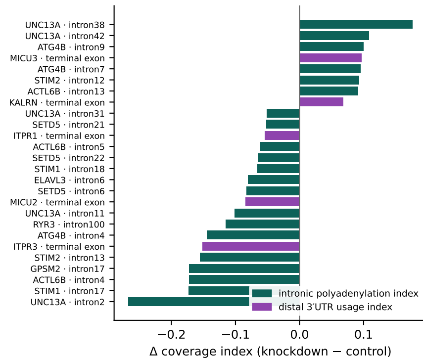
B · Alternative polyadenylation in \text{Ca}^{2+} genes, SH-SY5Y
