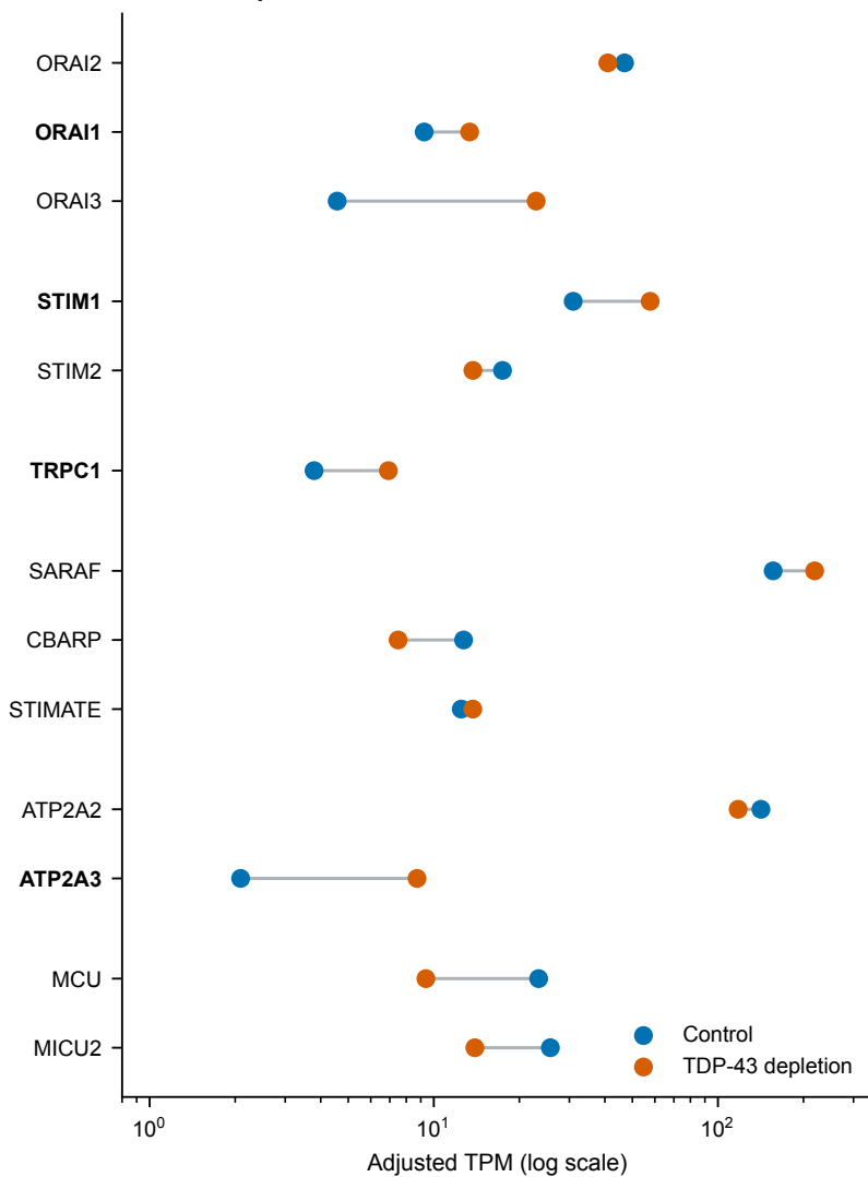
A Transcript abundance
