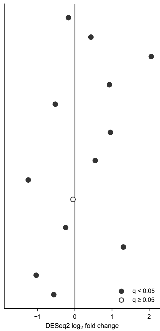
B Differential expression
