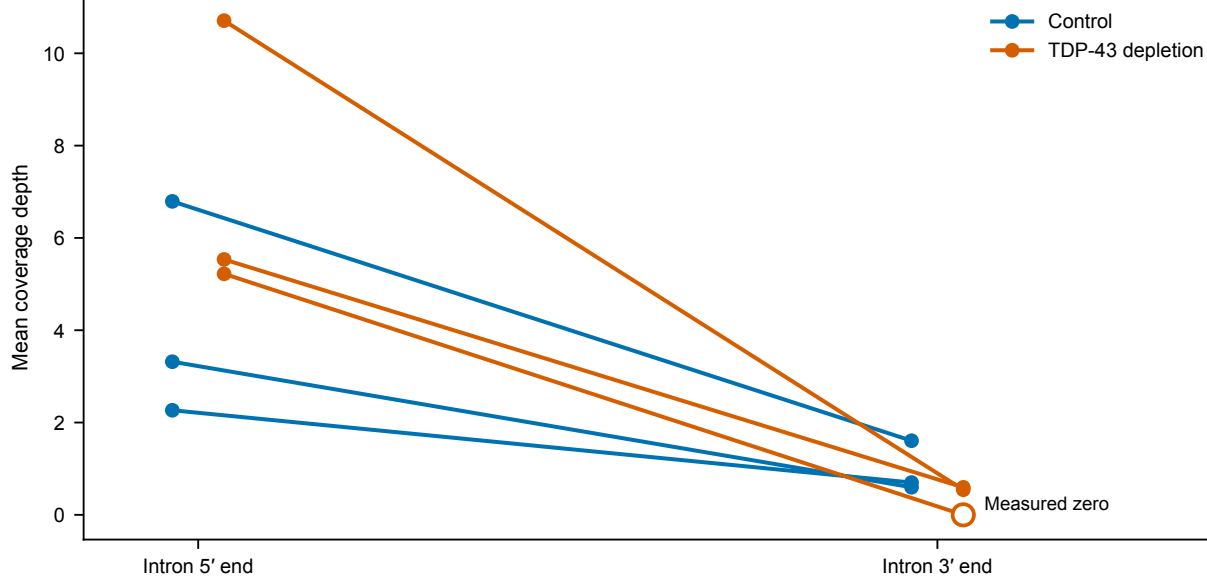
B STMN2 intron 2 positive control
