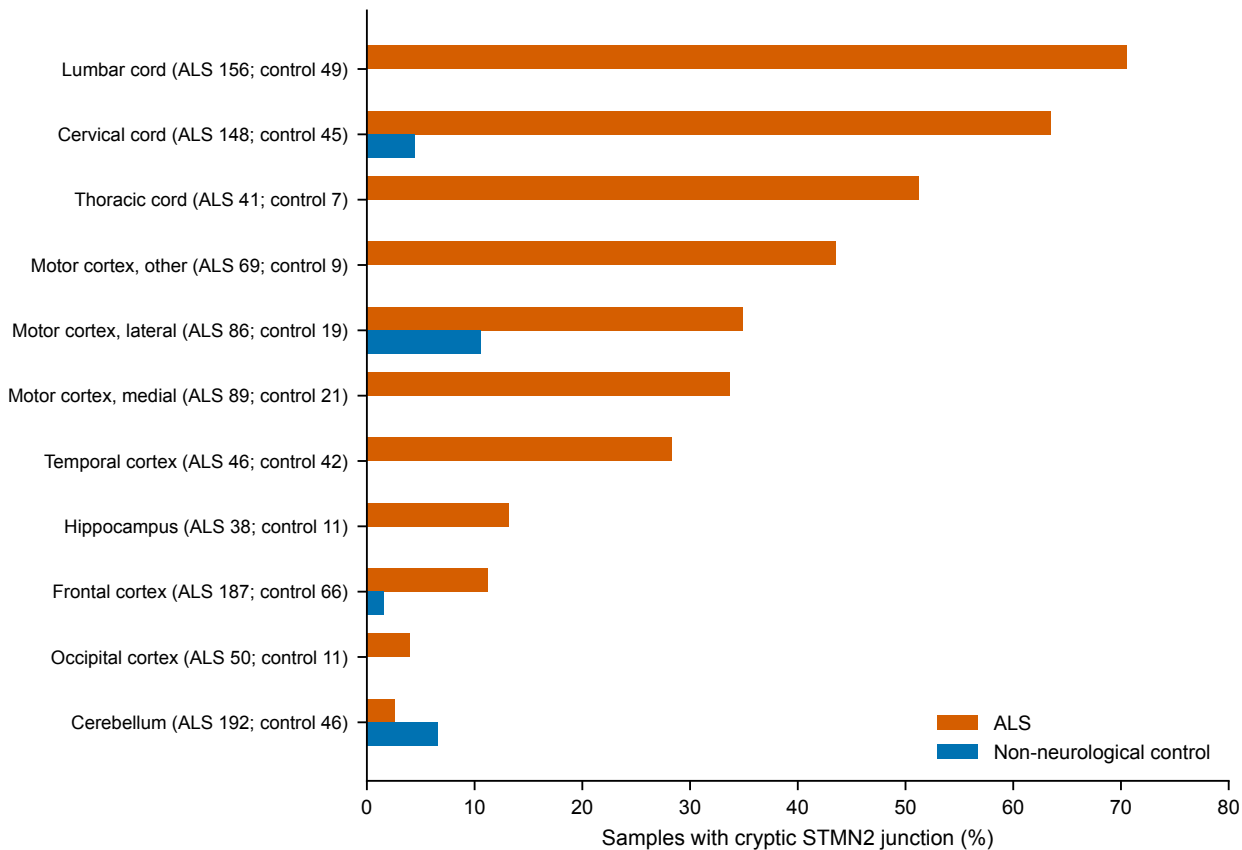
B gene-level STMN2
