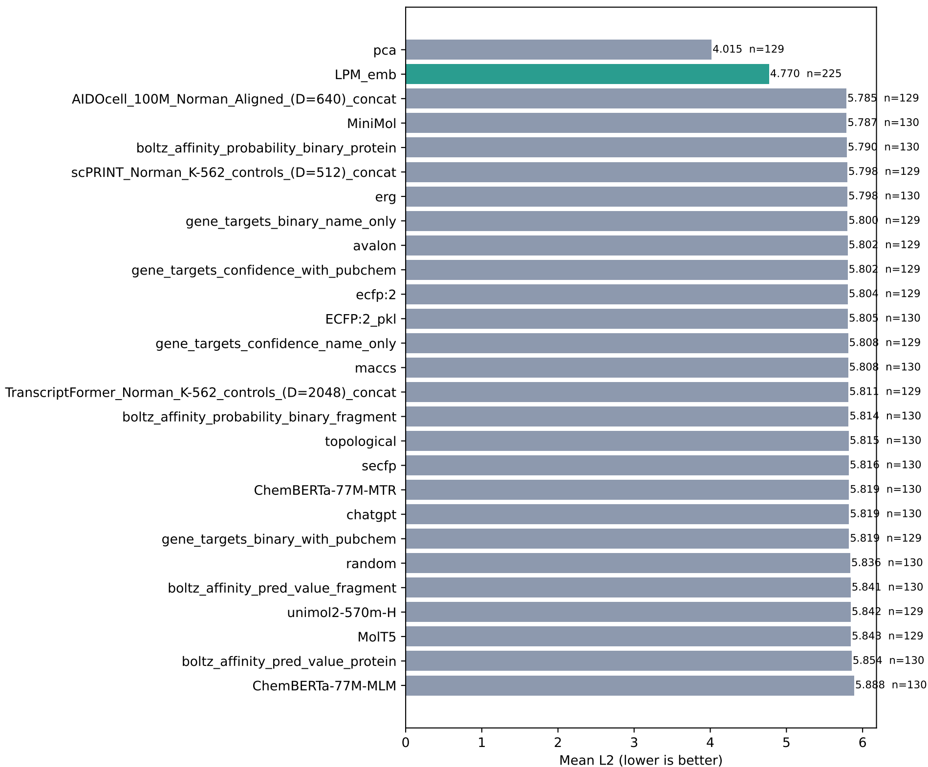
Tahoe LFC KNN restricted current results
