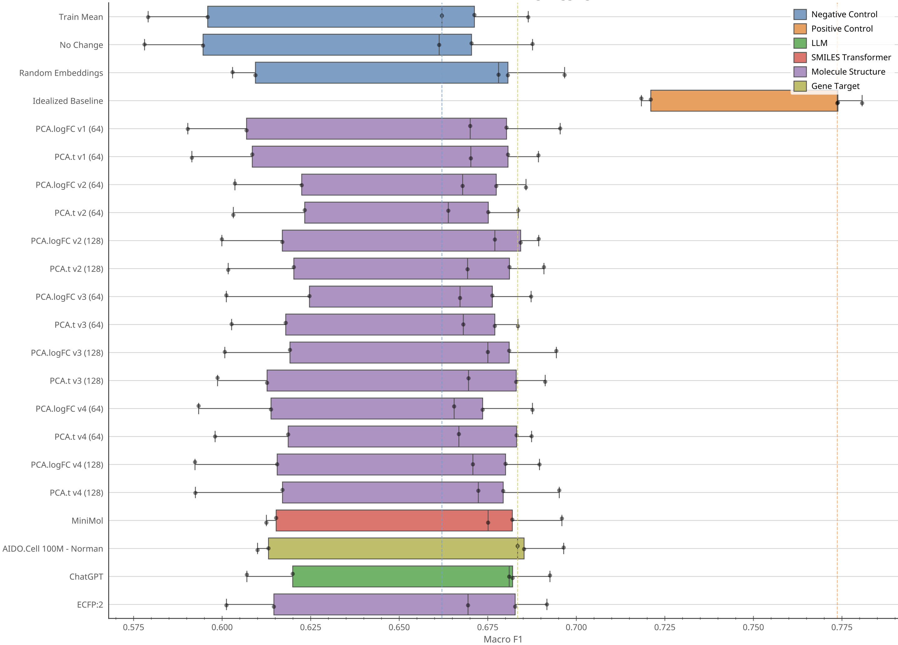
Tahoe DEG (PCA Embeddings, Aggregate)
