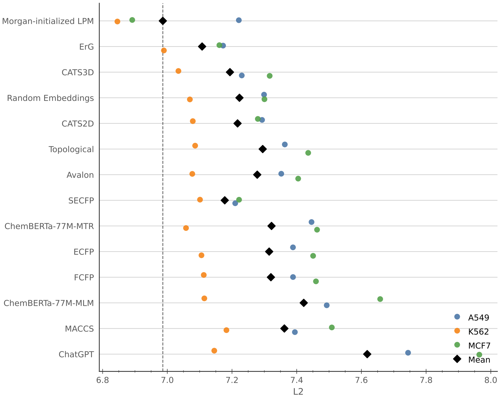
SciPlex LFC Heldout Molecules (KNN)
