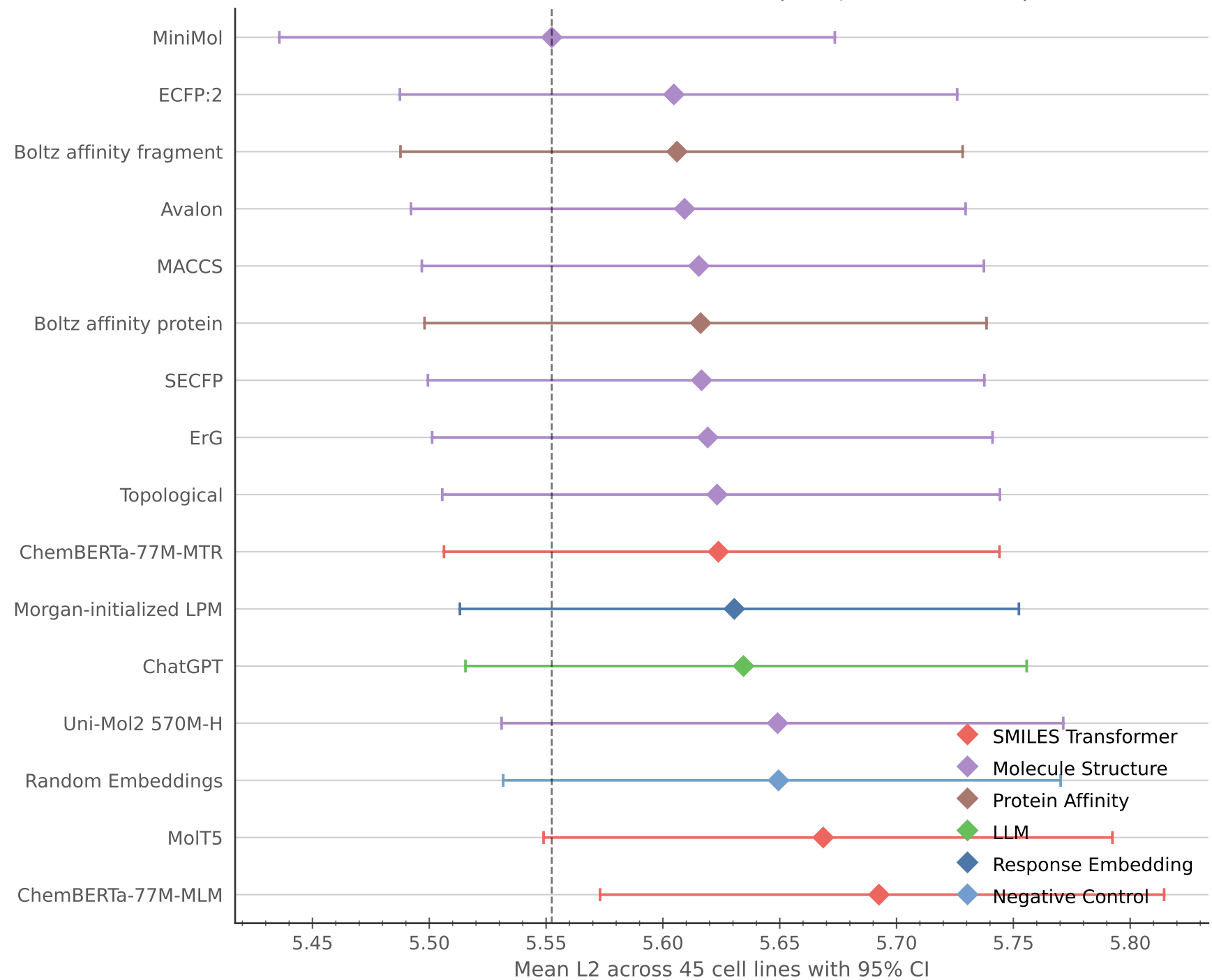
Tahoe LFC Heldout Molecules (KNN, PCA excluded)
