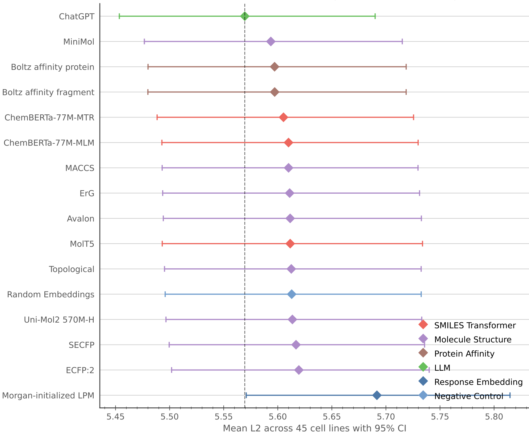
Tahoe LFC Heldout Molecules (LASSO, PCA excluded)
