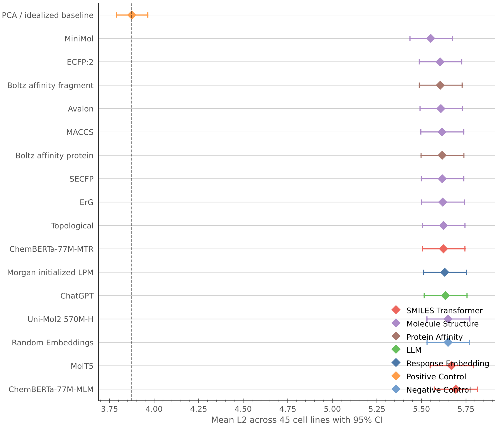
Tahoe LFC Heldout Molecules (KNN, PCA included)
