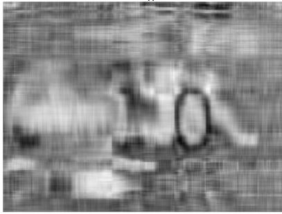
Rank-9 approx.
