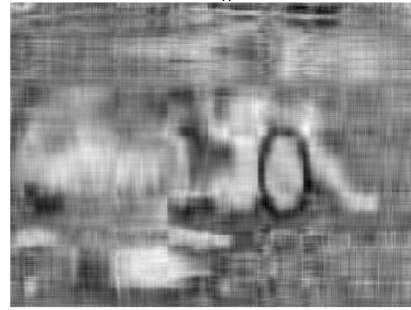
Rank-10 approx.
