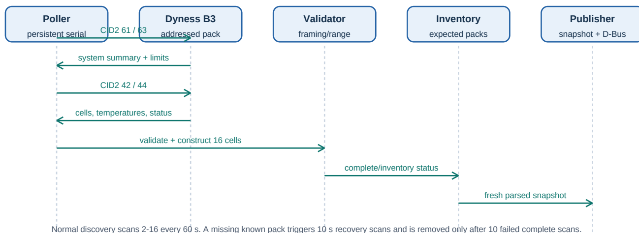
Figure 2 - RS485 polling, validation, inventory, and publication sequence.
