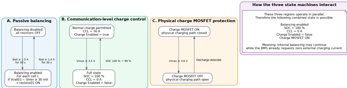
Dyness BMS Algorithm as Parallel UML State Machines Software version 2.50-71.10.11
