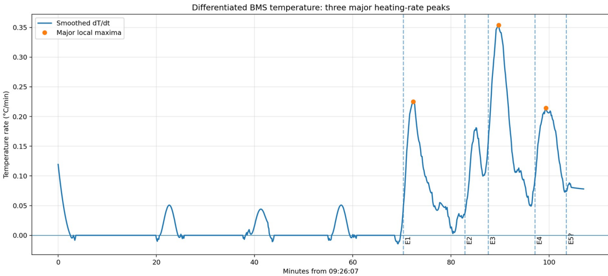
Figure 4. Smoothed derivative of BMS temperature. Local increases in heating rate identify changes in internal dissipation.
