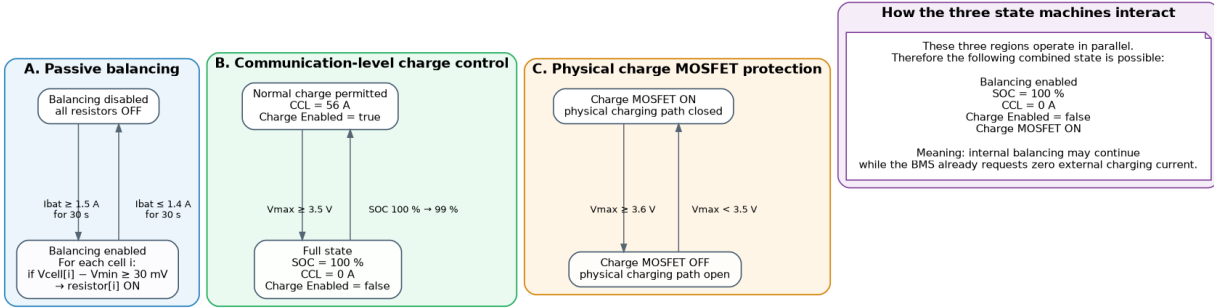
Figure 1. UML state-machine view of the three parallel control layers: passive balancing, communication-level charge control and physical charge-MOSFET protection.
