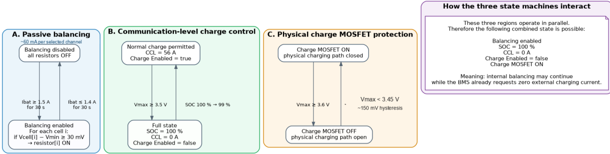
Figure 1. UML state-machine view of the three parallel control layers: passive balancing (approximately 60 mA per selected cell), communication-level charge control and physical charge-MOSFET protection, with reset below approximately 3.45 V.
